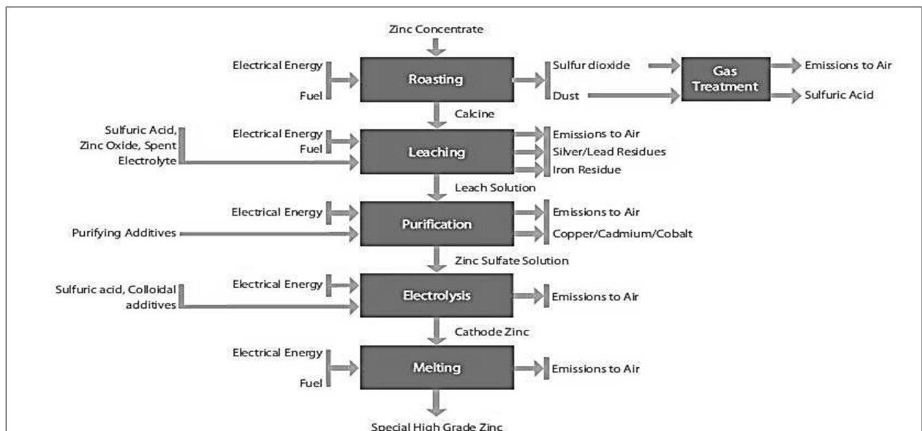
Hydrometallurgy of zinc extraction
